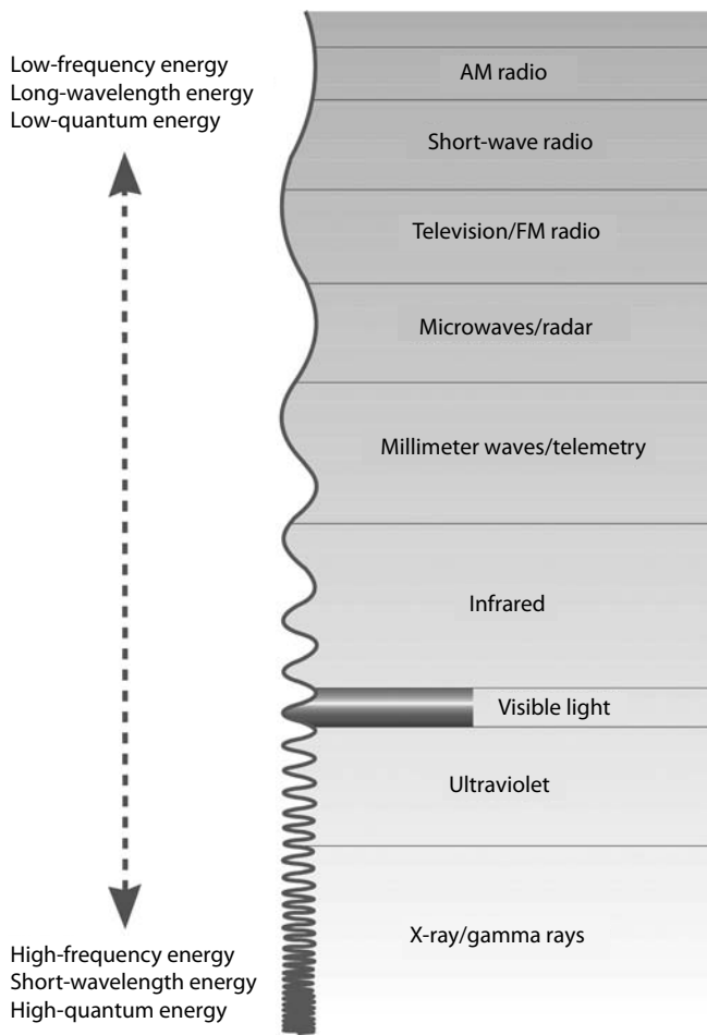
FIGURE 10.5 Electromagnetic spectrum.
