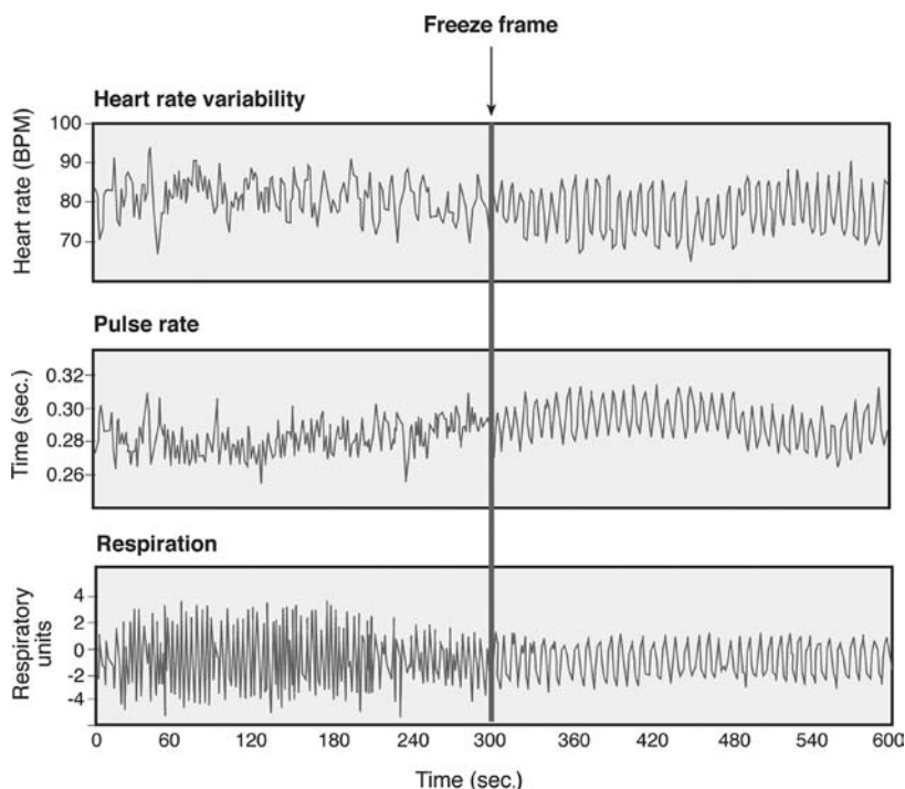
FIGURE 5.2 HeartMath entrainment.
